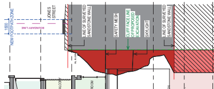
9 SECTION THROUGH CLIFF FACE
