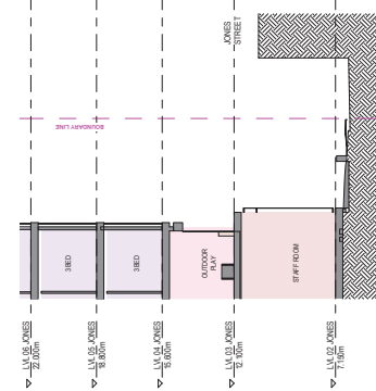
2 SECTION THROUGH CLIFF FACE
