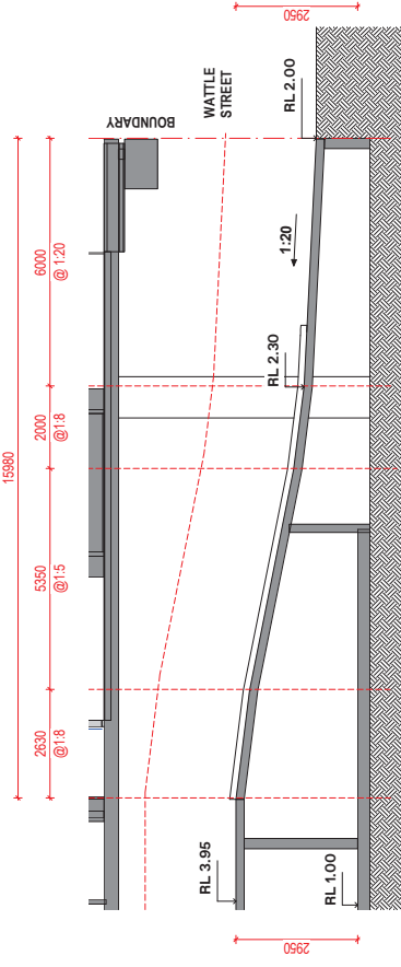
4 WATTLE STREET RAMP LEVEL 01
