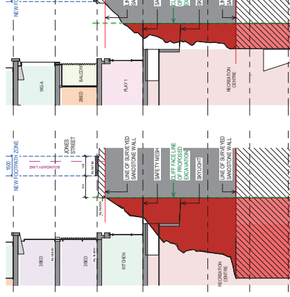
5 SECTION THROUGH CLIFF FACE
