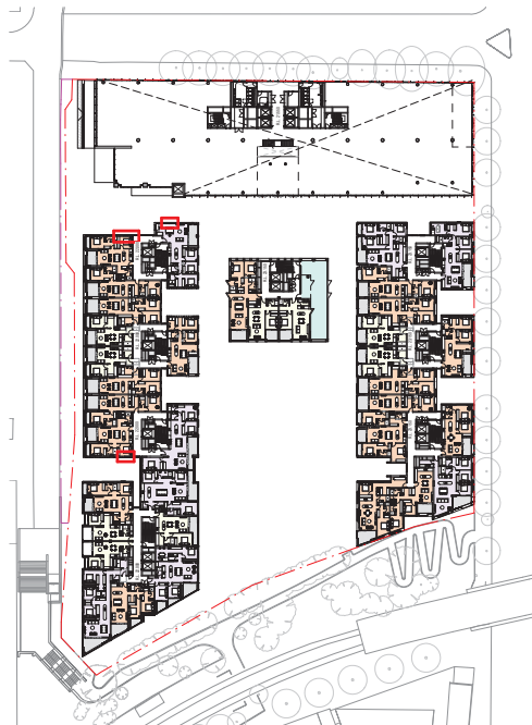
7 PRIVACY DETAIL C - LOCATION PLAN SCALE: 1 : 500
