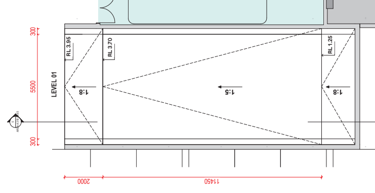
3 WATTLE STREET RAMP LEVEL 00 UP TO LEVEL 01
