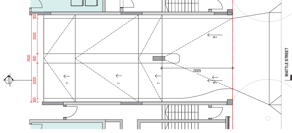
2 CARPARK RAMP LEVEL 01 DOWN TO LEVEL 00
