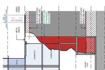
9 SECTION THROUGH CLIFF FACE
